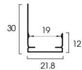
CHY-2 aluminium profile with glare shield
