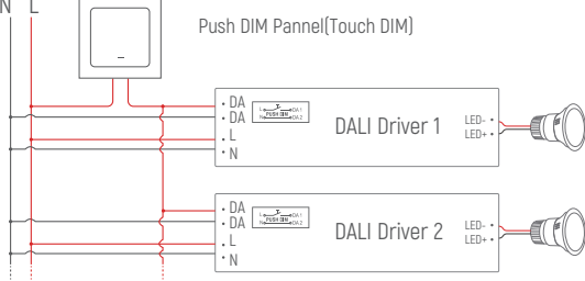
Push DIM(Touch DIM) Diagram
