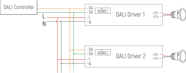
DALI Wiring Diagram
