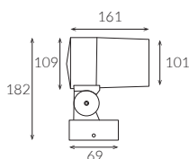
Adjustable Optic
