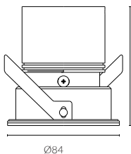
Fixed Optic
