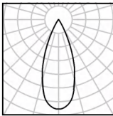
8.7W Ra98 3000K 36° Curve Baffle
