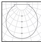
12W Ra98.3000K 120°
