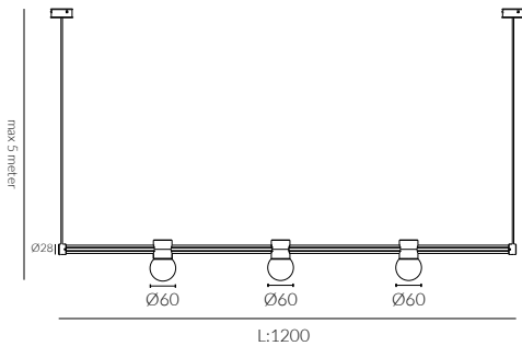
Fixed Optic
