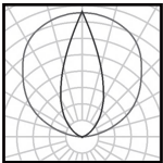
22W Ra92 3000K Asymmetric Uplight Distribution
