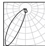
25W Ra92 3000K Asymmetrical
